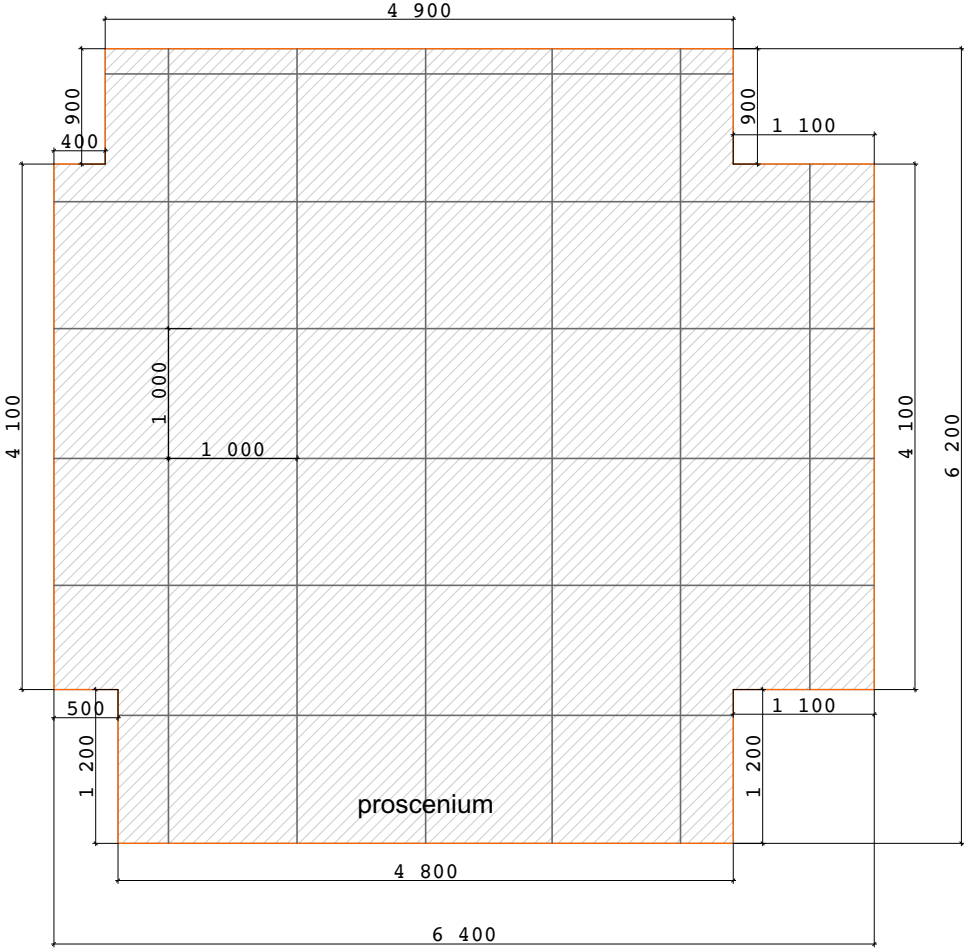
Stage dimensions h - 0.4m
